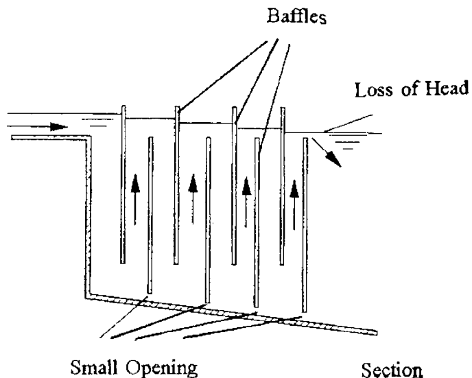
Figure 2. A simple flocculator
